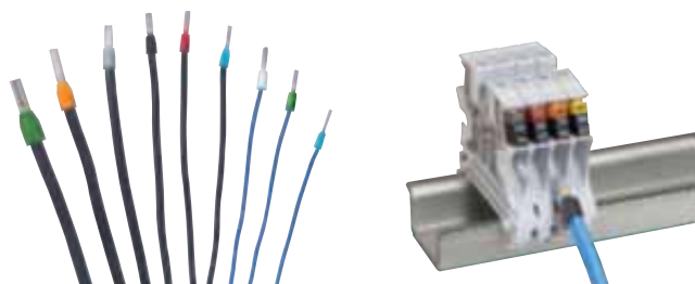
Example of different wires and ferrules
