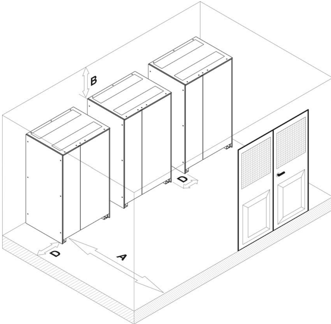
Picture 5 – Minimum distances from the walls
