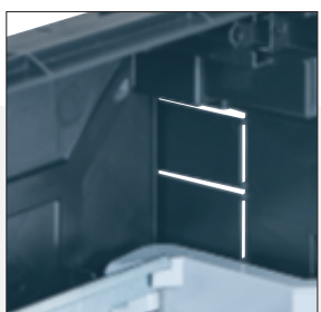
6 CABLE ENTRIES Cut-out entries all around the box for feeding through cables or trunking.
